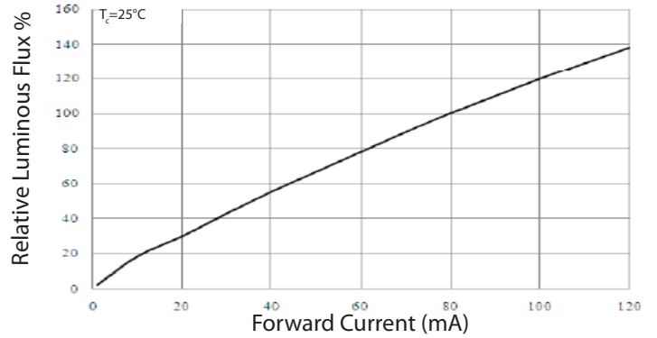
I_f ---- Relative Luminous flux
