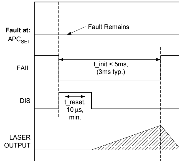
Unsuccessful Fault Reset Attempt
