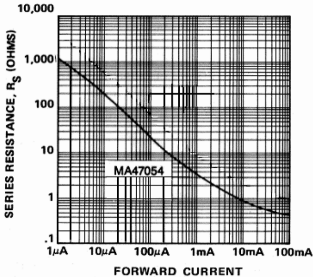
Typical R_s vs. I_F @ T_{AMB} = +25^\circ\text{C}
