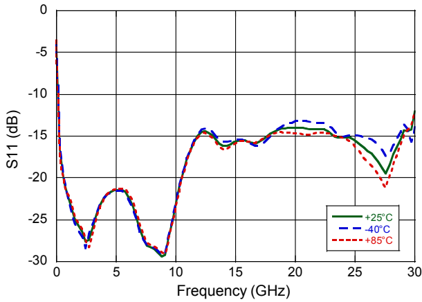
Low Frequency S-Parameters
