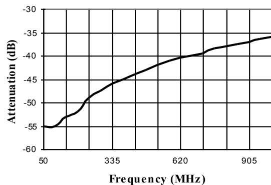
Attenuation vs. Frequency @ Control Voltage = 0V
