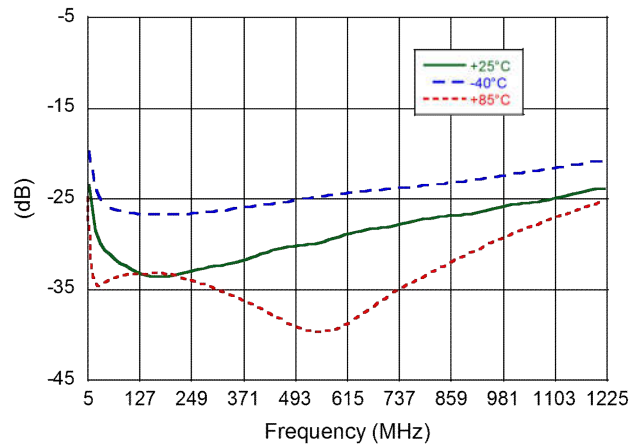
Isolation (pin 3 - 5)
