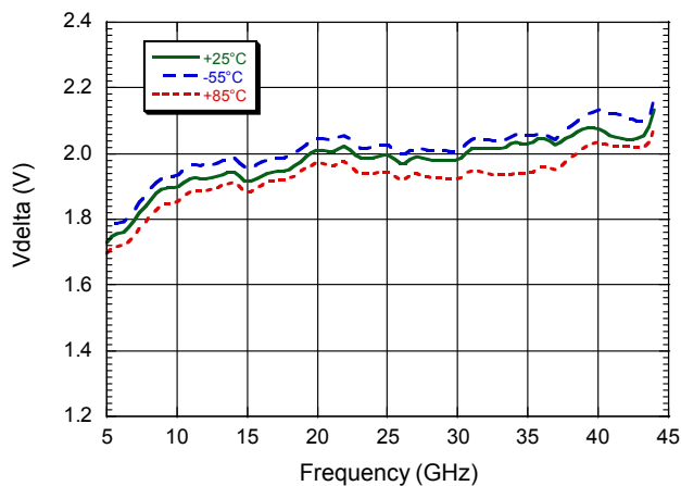
Vdelta vs. Frequency, P_{IN} = +15 dBm
