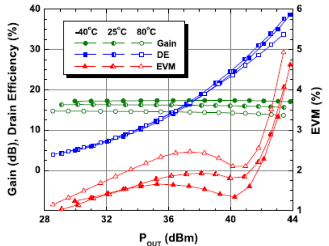
Drain Efficiency, Gain, & EVM 28 V, 600 mA, 2500 MHz
