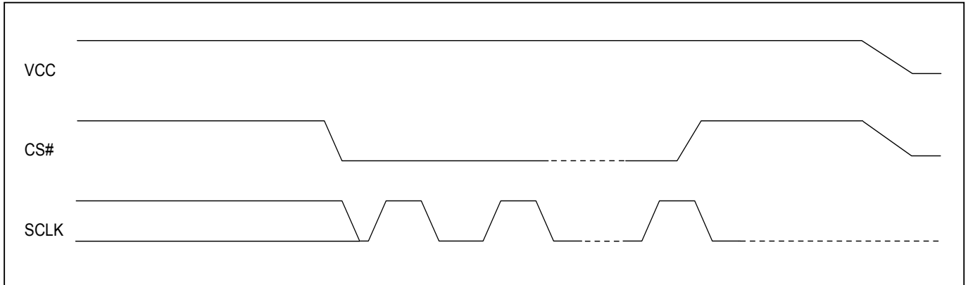
Figure 33. Power-Down Sequence
