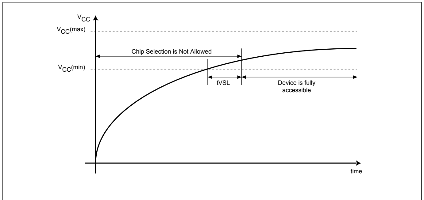
Figure 34. Power-up Timing
