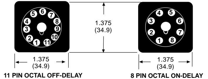
11 PIN OCTAL OFF-DELAY
