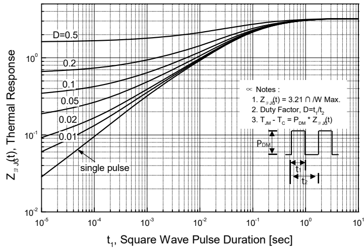
Figure 11-2. Transient Thermal Response Curve for SLF7N60C
