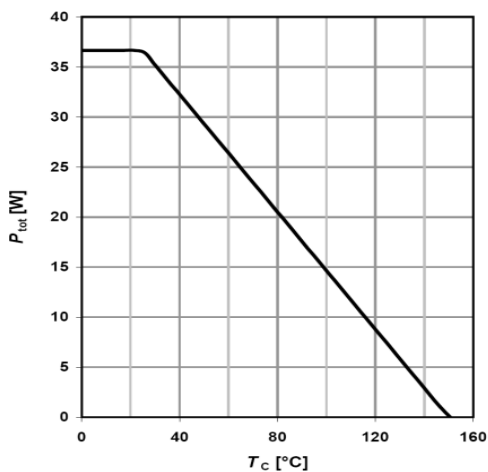
Figure 3: Power Dissipation(TO-220,TO-252)
