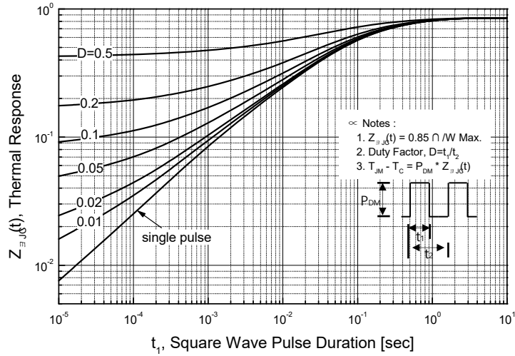
Figure 11-1. Transient Thermal Response Curve for SLP8N60C
