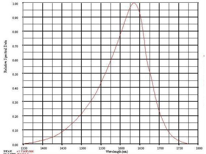
SPECTRAL OUTPUT
