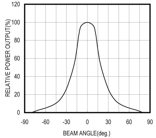
RADIATION PATTERN
