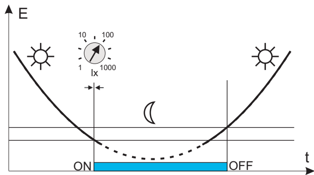
Fig. 3.: Diagrams of the operation principles of the TS-41-3 TWILIGHT SWITCH.
