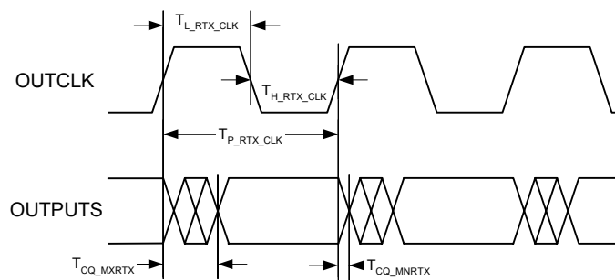
Figure 53: SNI Rising Edge Transmit Timing
