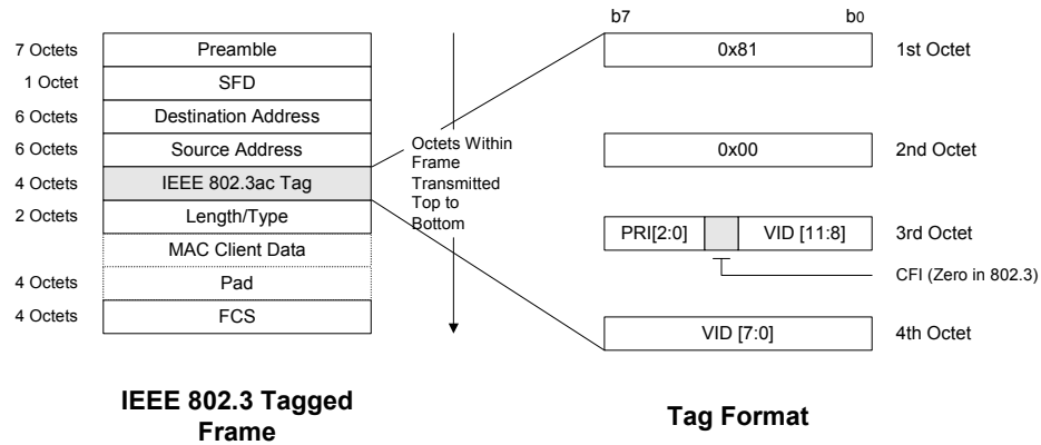
Figure 24: IEEE Tag Frame Format
