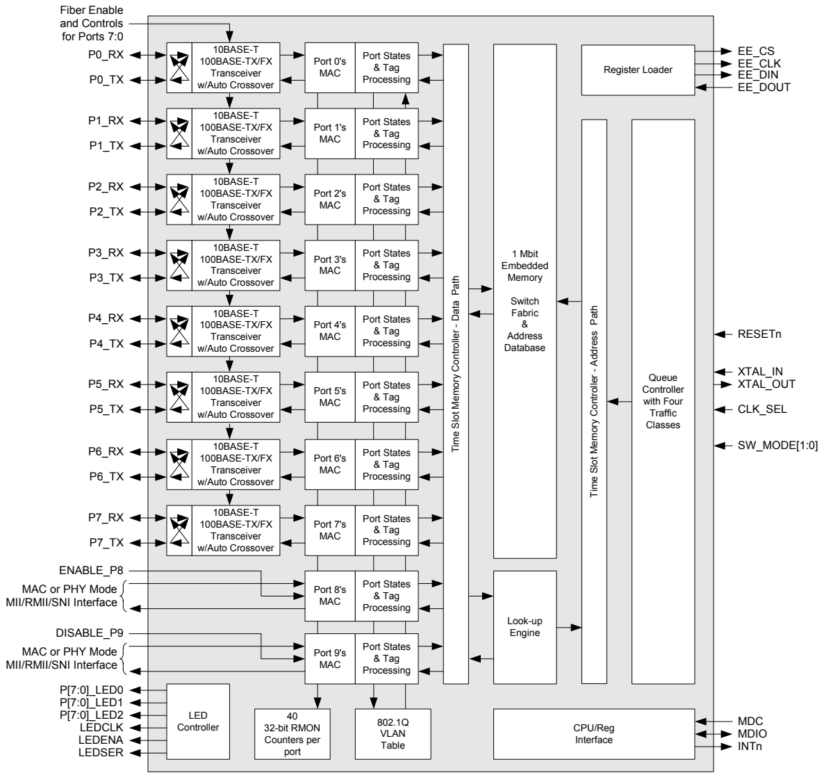
88E6083 Top Level Block Diagram
