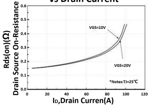
On-Resistance Variation vs Drain Current
