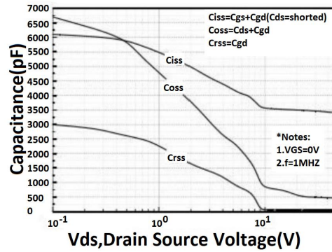
Capacitance Characteristics
