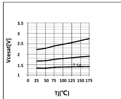
Saturation Voltage vs. Case Temperature at Vaian Current Level
