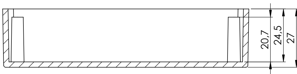
SECTION B-B
