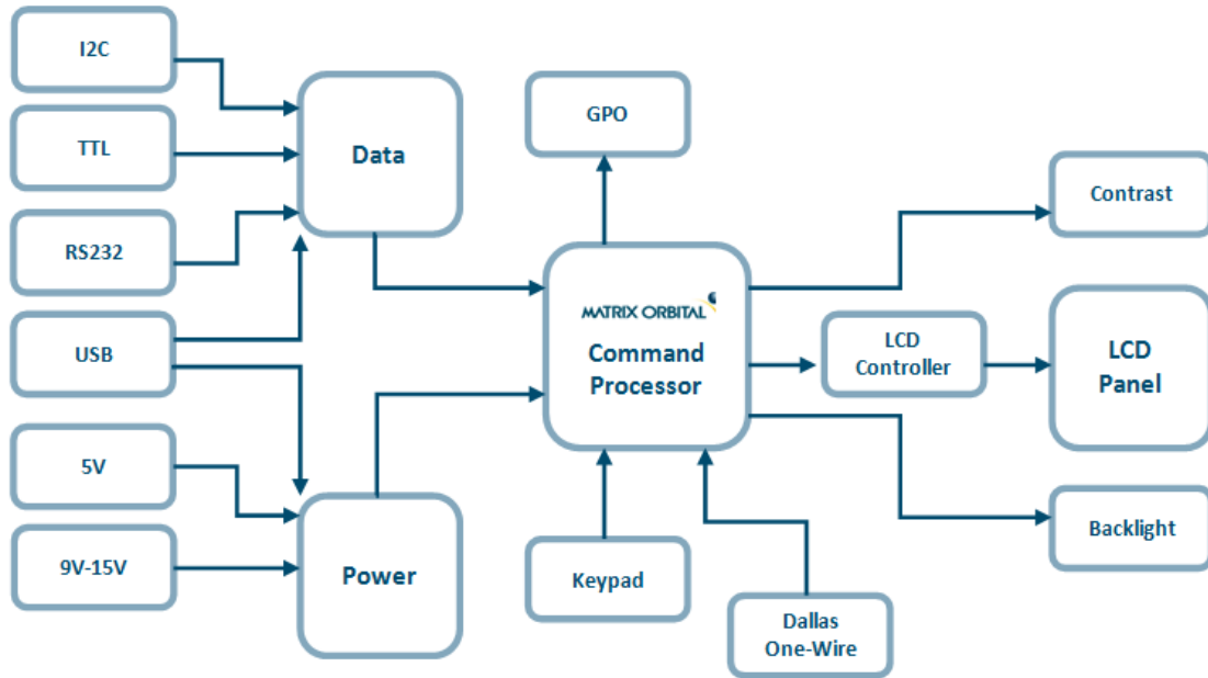
Figure 17: Functional Diagram
