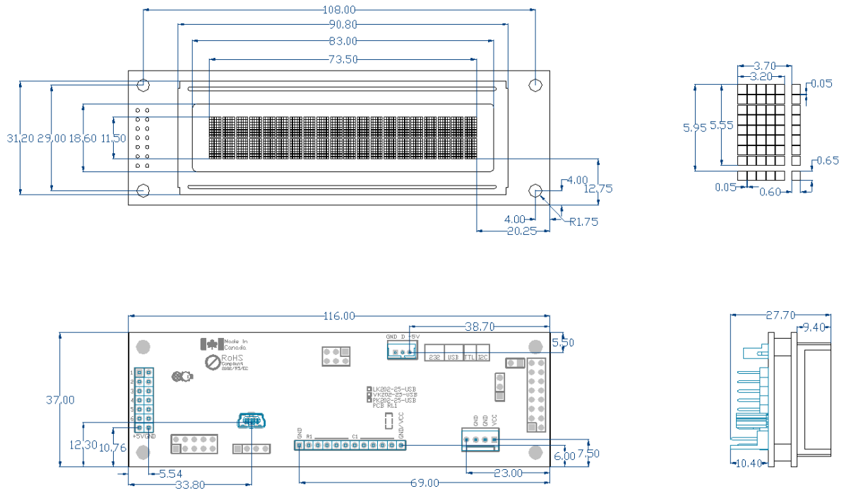
Figure 19: LK202-25-USB Dimensional Drawing
