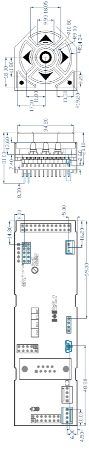
Figure 20: USB Model Drawing
