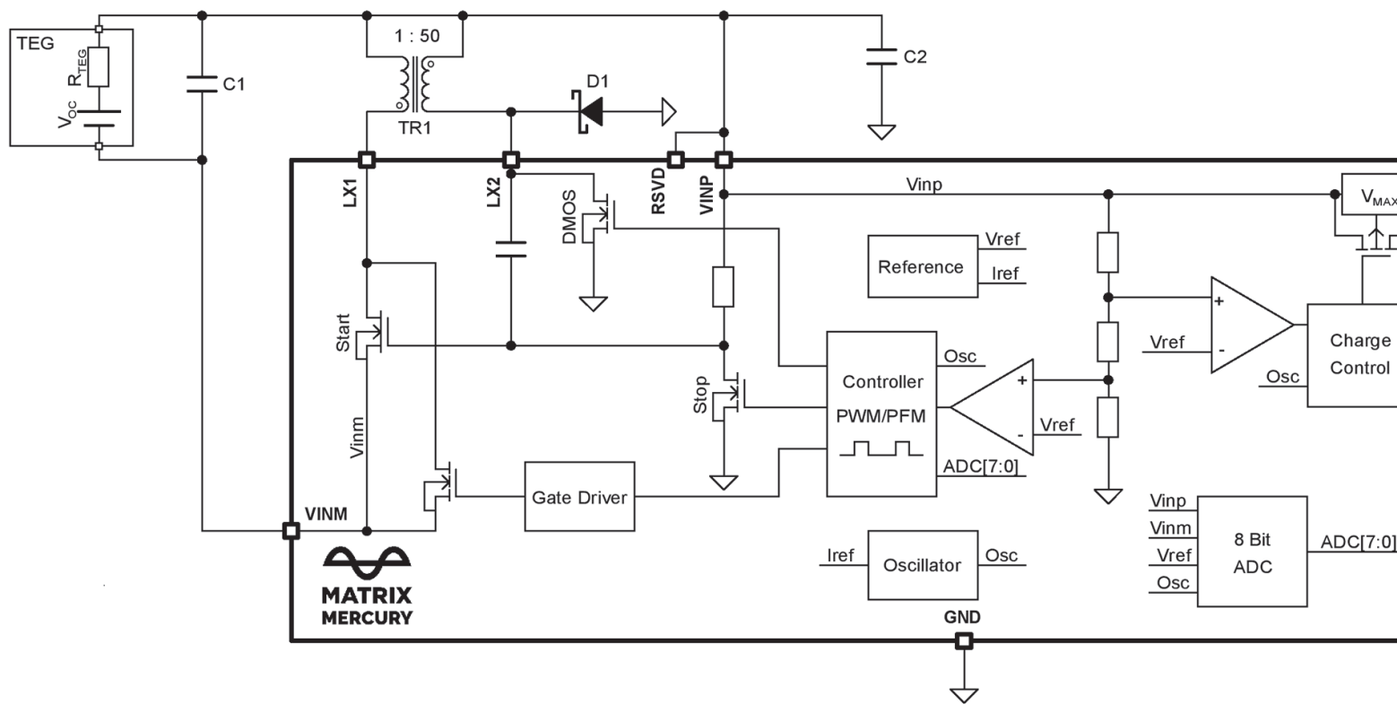
Figure 5: Block Diagram
