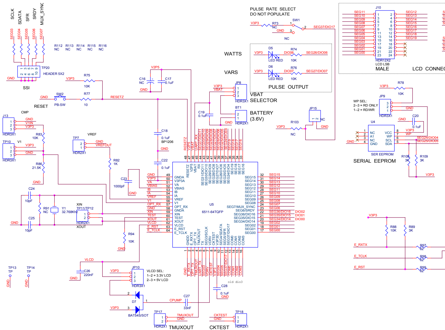
Figure 4-3: 71M6511 4-Layer Demo Board: Electrical Schematic 3/3
