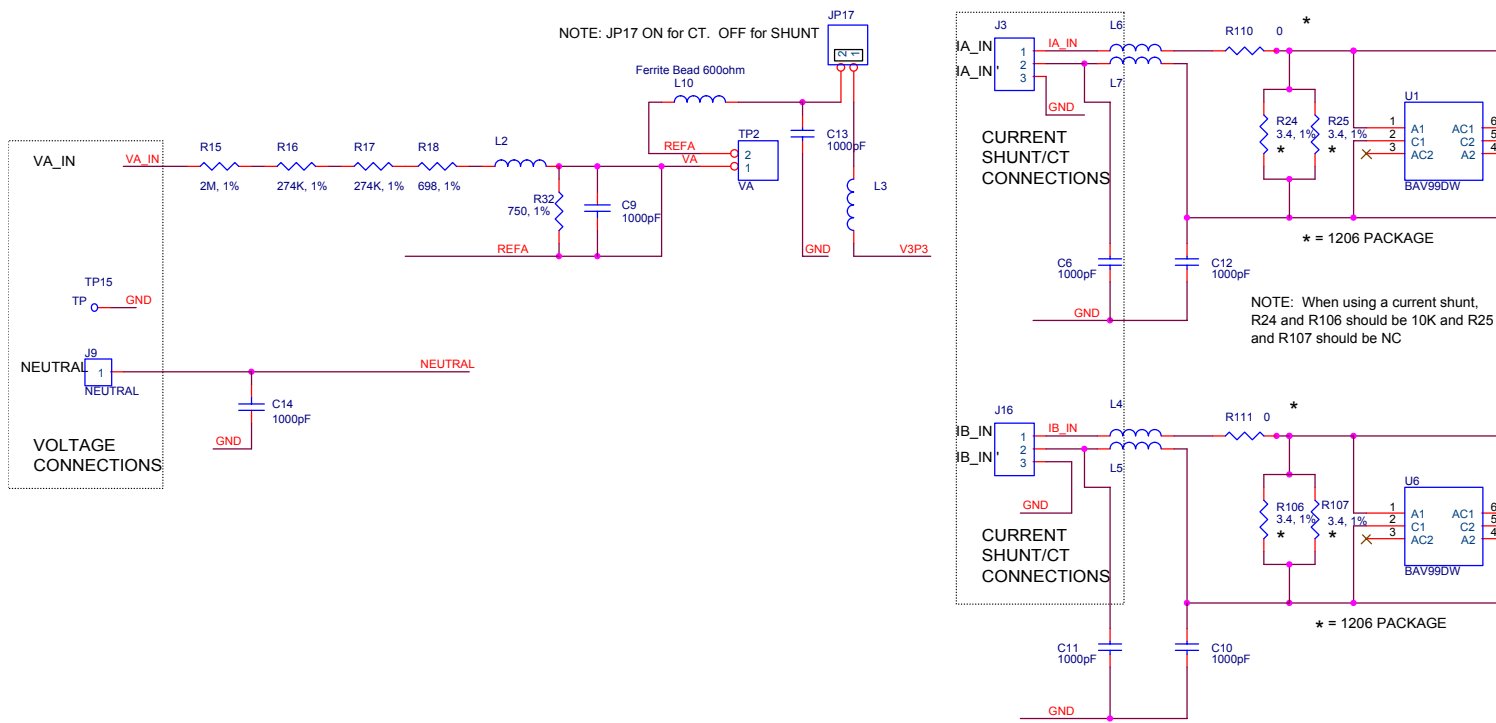
Figure 4-8: 71M6511 2-Layer Demo Board (Transformer Power Supply): Electrical Schematic 2/3
