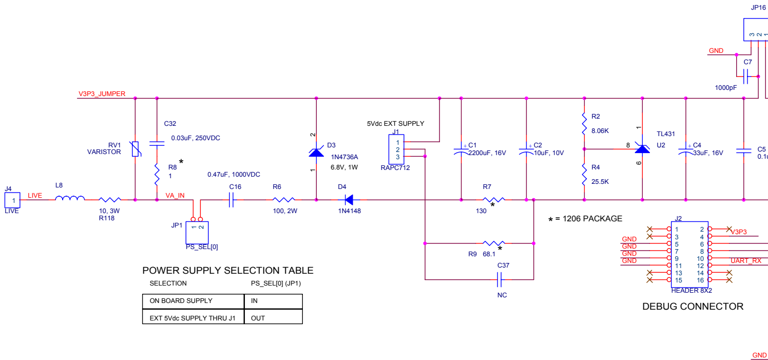
Figure 4-4: D6511T4A8 2-Layer Demo Board (Capacitive Power Supply): Electrical Schematic 1/3
