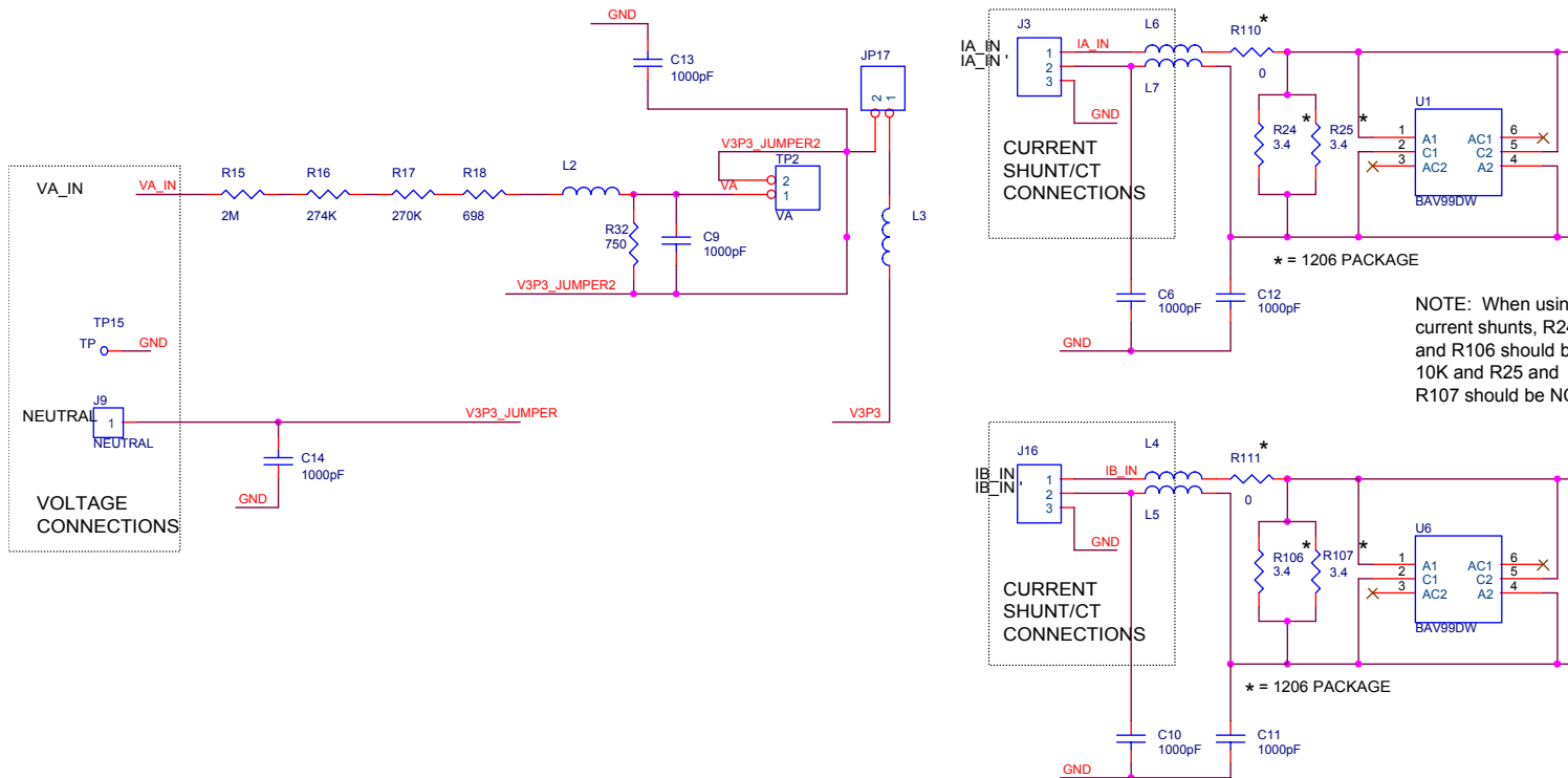
Figure 4-5: D6511T4A8 2-Layer Demo Board (Capacitive Power Supply): Electrical Schematic 2/3
