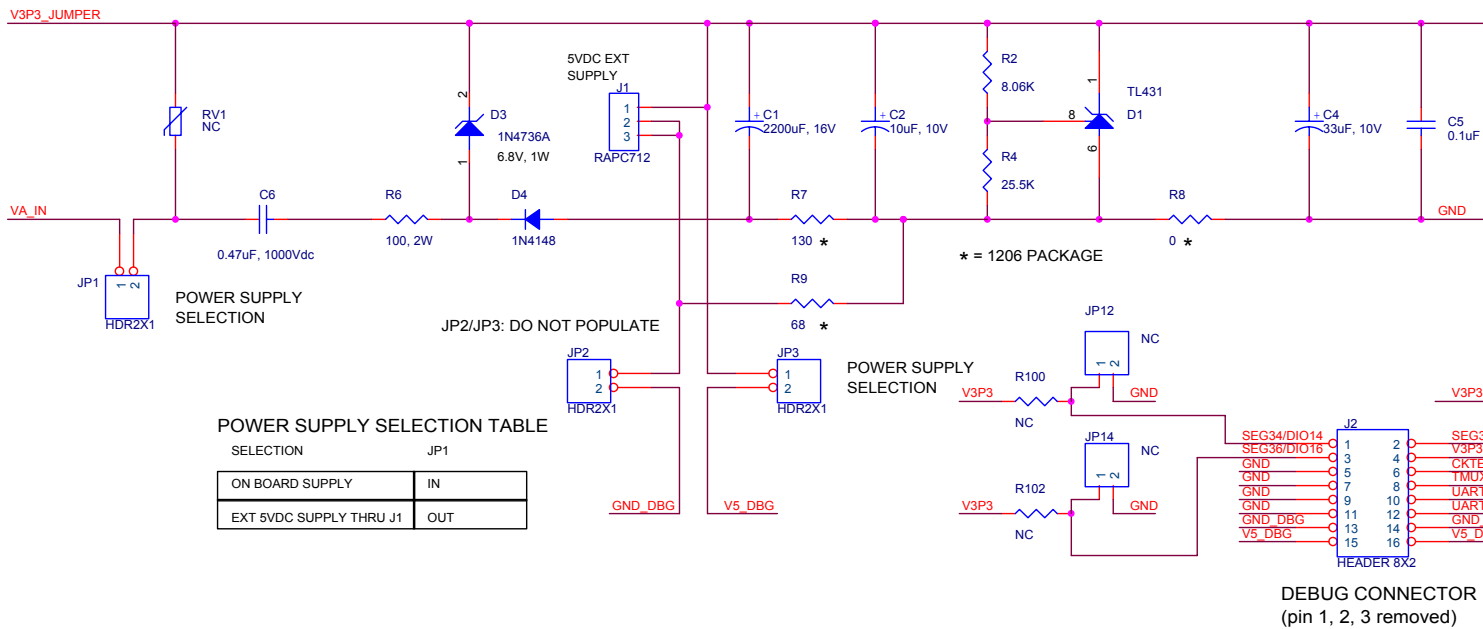
Figure 4-1: 71M6511 4-Layer Demo Board: Electrical Schematic 1/3
