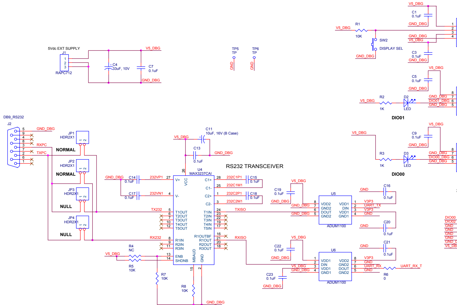
Figure 4-25: Debug Board: Electrical Schematic
