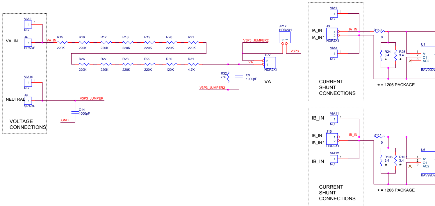
Figure 4-2: 71M6511 4-Layer Demo Board: Electrical Schematic 2/3
