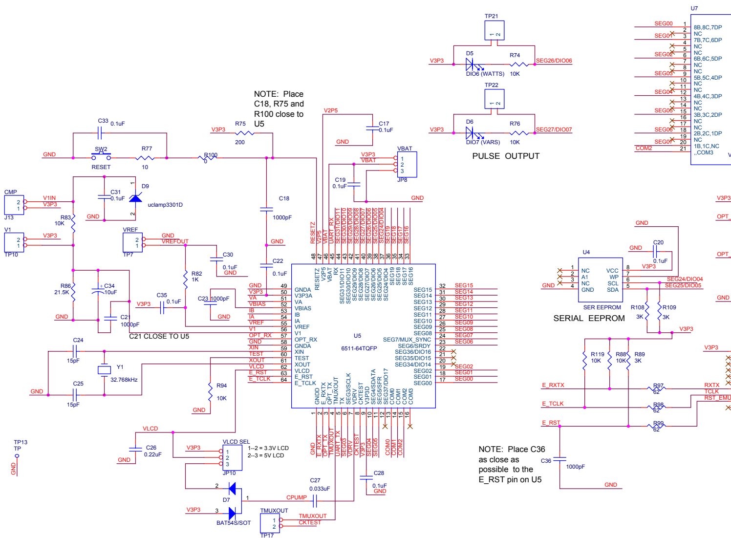
Figure 4-6: D6511T4A8 2-Layer Demo Board (Capacitive Power Supply): Electrical Schematic 3/3
