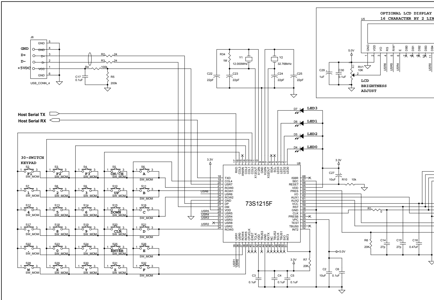
Figure 26: 73S1215F Typical Application Schematic
