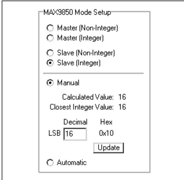
Figure 9. Slave (Integer) Mode
