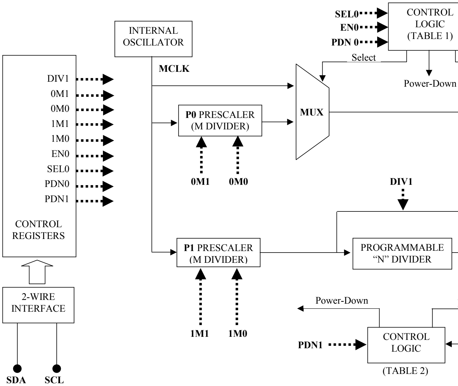
BLOCK DIAGRAM DS1077L Figure 1
