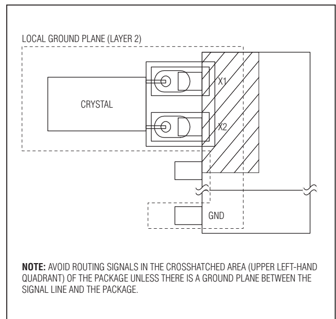
Figure 2. Layout Example
