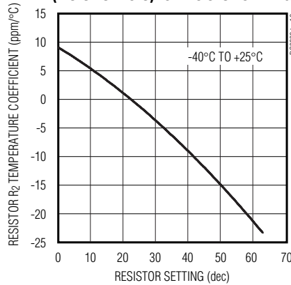
RESISTOR R_2 TEMPERATURE COEFFICIENT (-40°C TO +25°C) vs. RESISTOR SETTING
