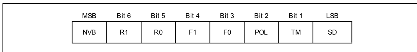
Figure 5. Configuration Register
