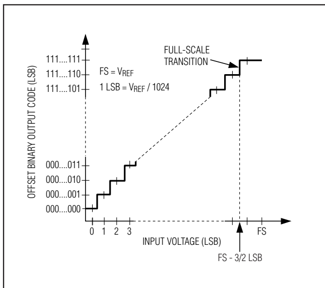
Figure 3. Unipolar Transfer Function—Full Scale (FS) = V_{\text{REF}}
