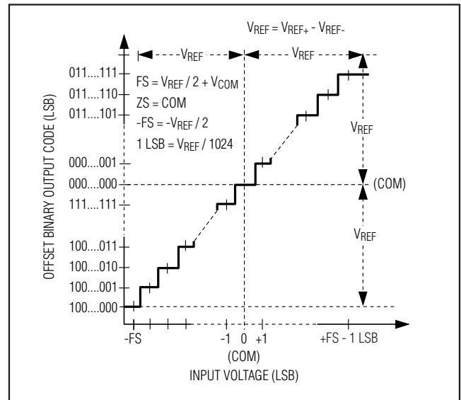
Figure 4. Bipolar Transfer Function—Full Scale ( \pm\text{FS} ) = \pm V_{\text{REF}} / 2
