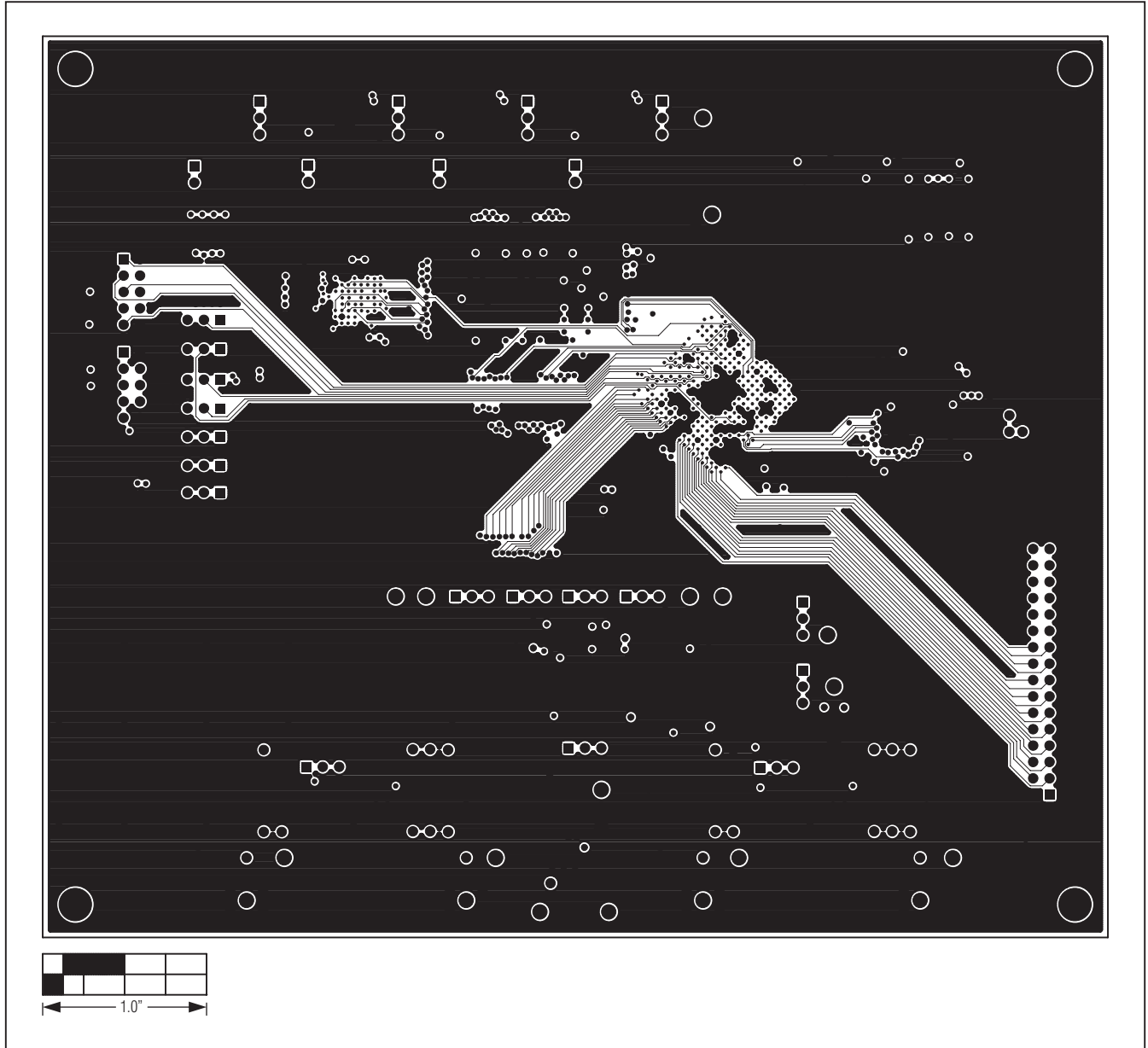
Figure 10. MAX11103 EV Kit PCB Layout—Layer 3
