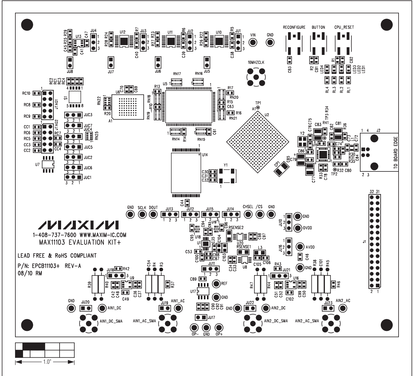
Figure 7. MAX11103 EV Kit Component Placement Guide—Top
