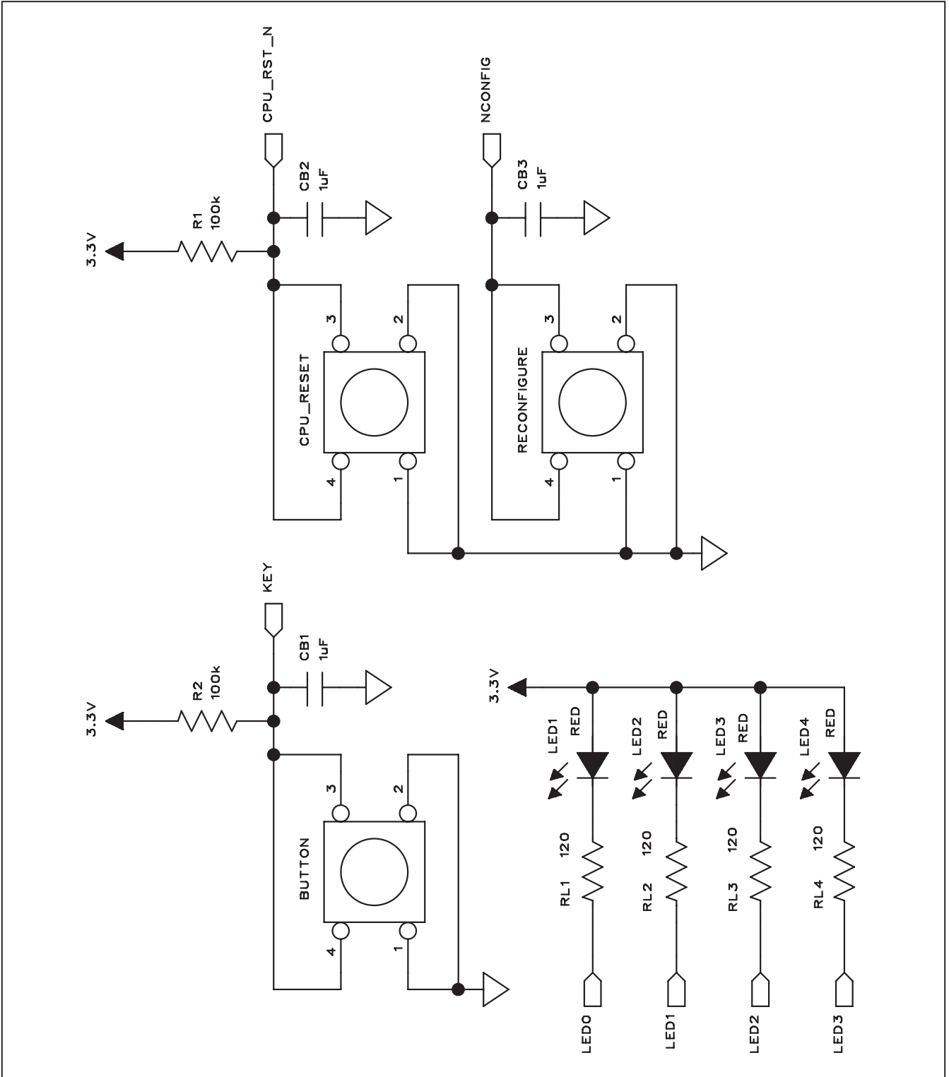
Figure 6g. MAX1105 EV Kit Schematic (Sheet 7 of 12)
