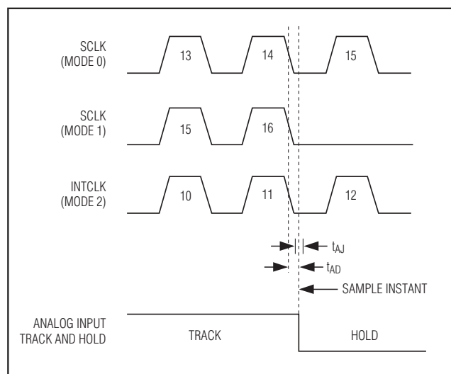
Figure 19. Aperture Diagram
