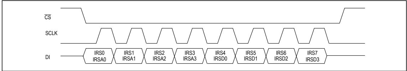
Figure 8. Serial Interface Data Input
