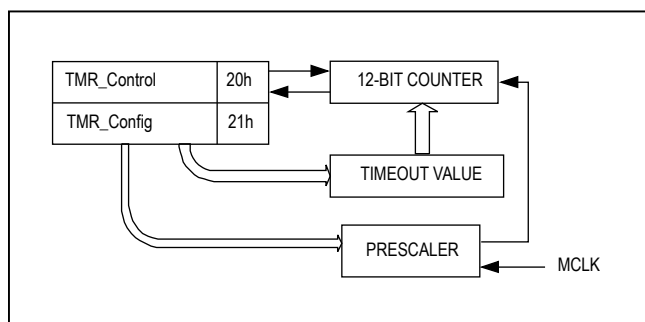
Figure 6. Timer Module
