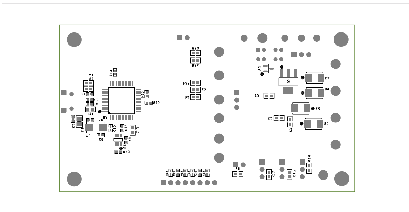
MAX14828 EV Kit—Bottom Silkscreen
