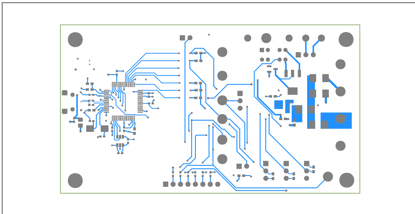
MAX14828 EV Kit—Bottom
