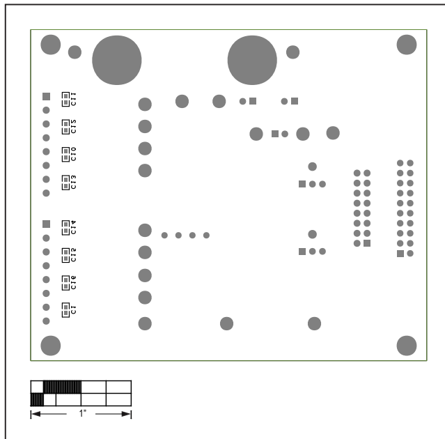
MAX14915 EV Kit—Bottom Silkscreen
