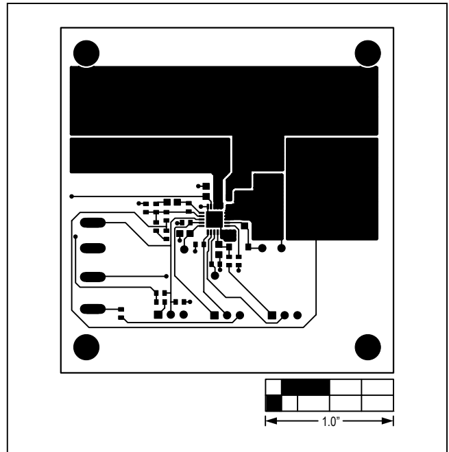
Figure 3. MAX15020 EV Kit PCB Layout—Component Side
