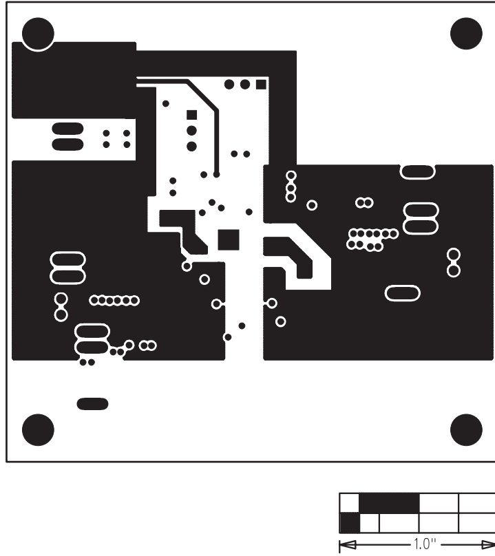
Figure 4. MAX15022 EV Kit PCB Layout—GND Layer 2
