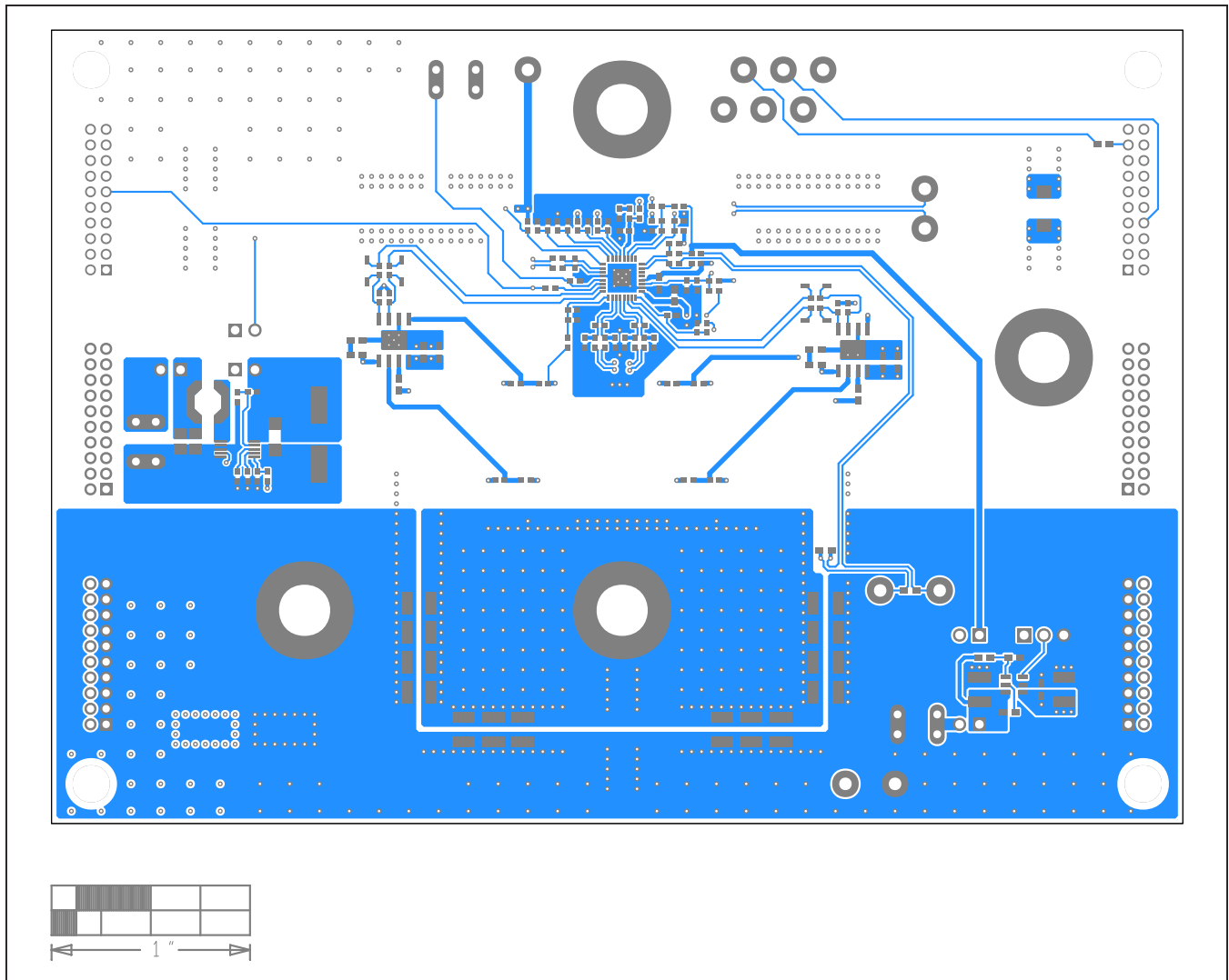
EV Kit PCB Layout—Bottom Layer
