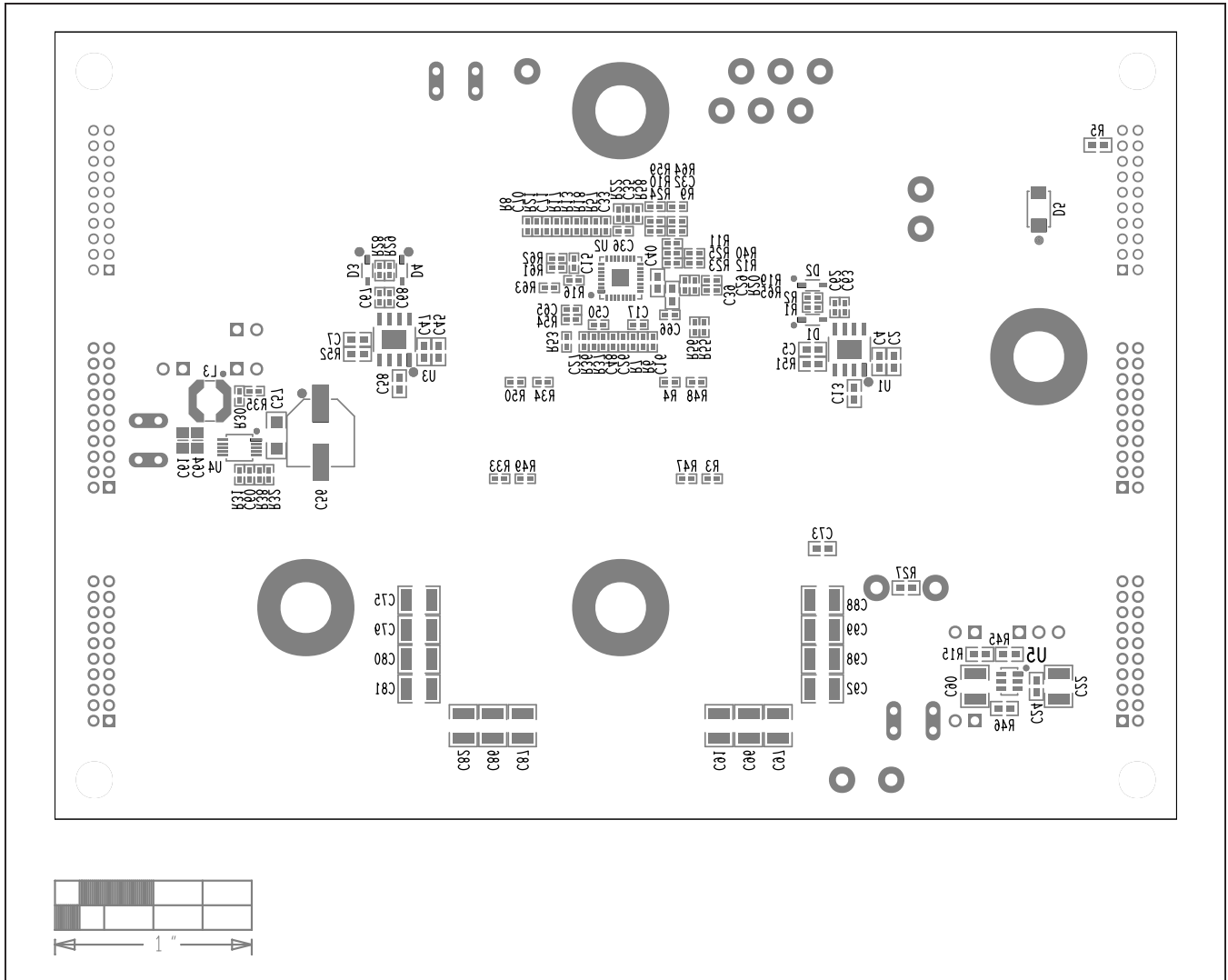
EV Kit Component Placement Guide—Bottom Silkscreen
