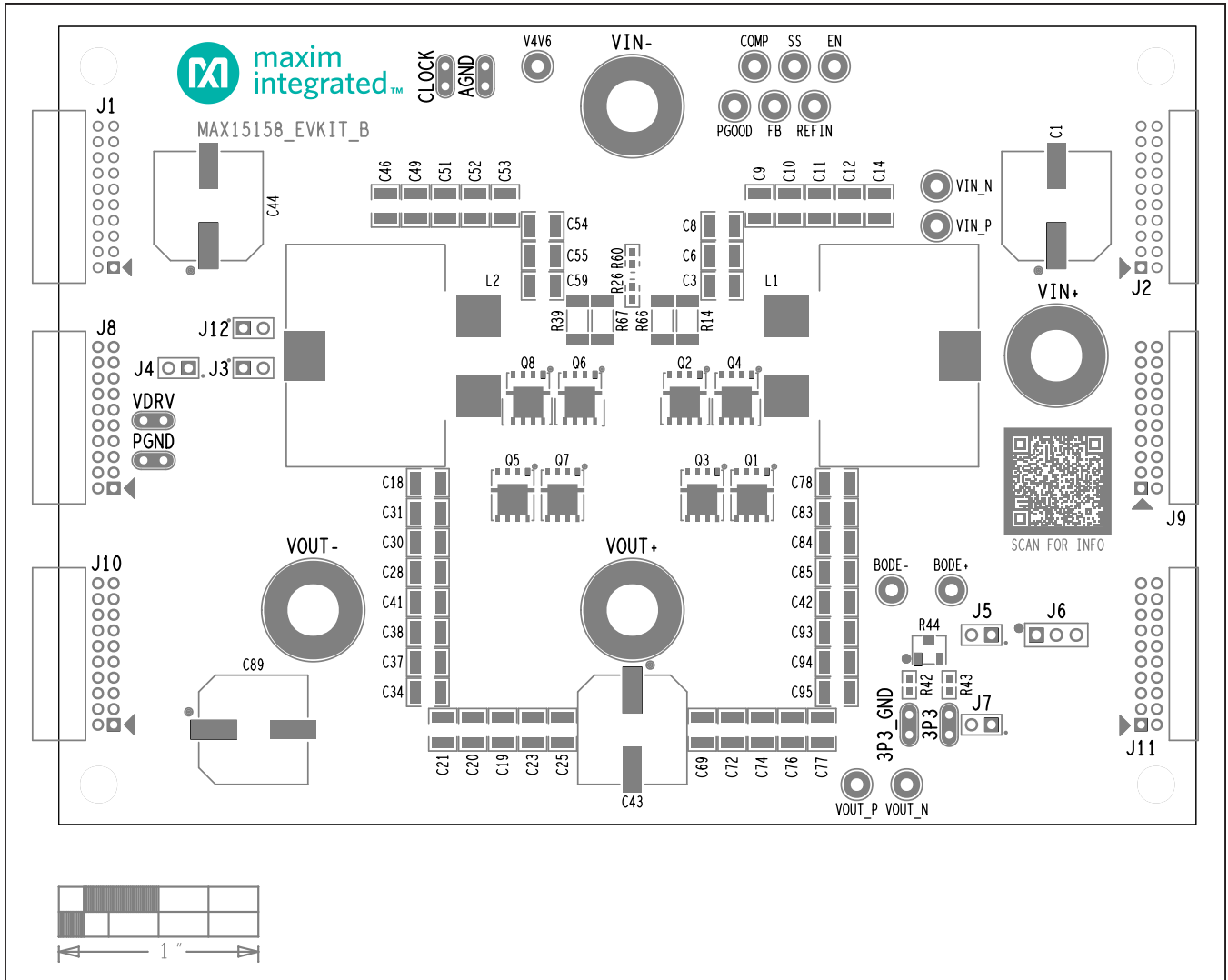
EV Kit Component Placement Guide—Top Silkscreen
