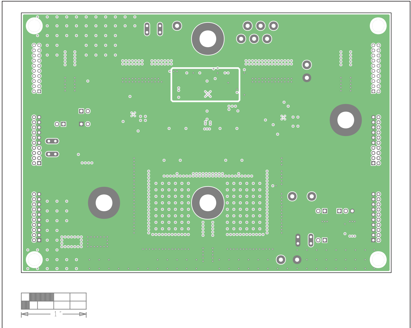
EV Kit PCB Layout—Internal Layer 3
