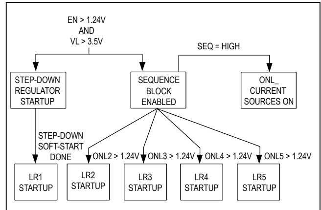
Figure 5. Startup Conditions
