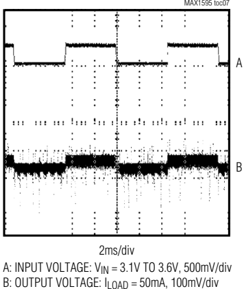
LINE-TRANSIENT RESPONSE
