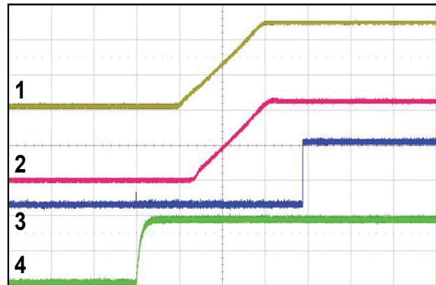
Startup Into Load, Controlled with VIN, 10Ω Resistive Load
