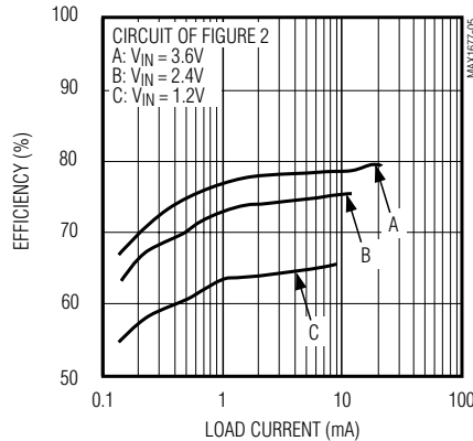
EFFICIENCY vs. LOAD CURRENT (LCD V_{OUT} = 20\text{V} )
