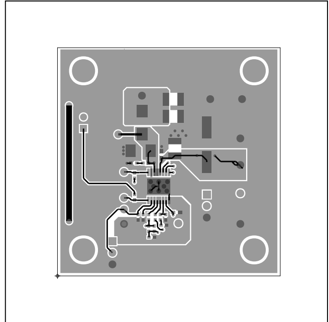
Figure 3. MAX16935 EV Kit PCB Layout—Component Side
