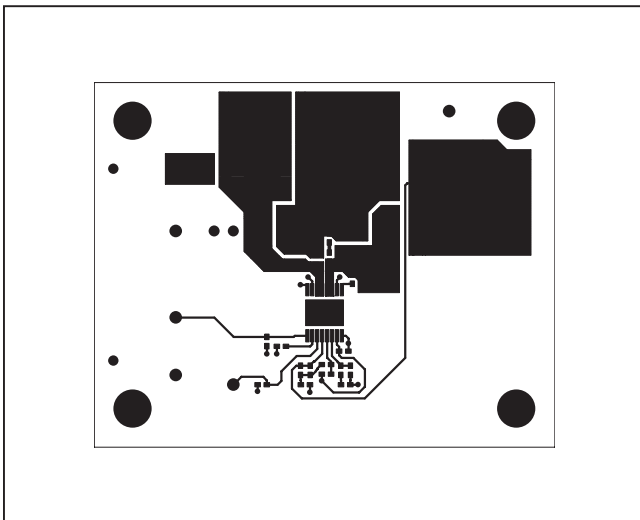
Figure 3. MAX16977 EV Kit PCB Layout—Component Side
