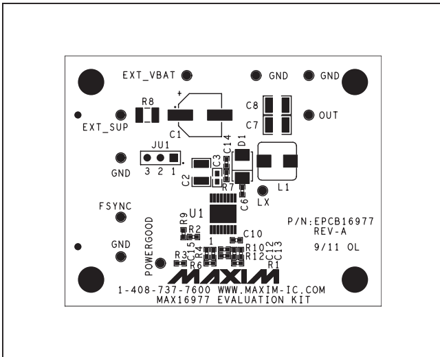
Figure 2. MAX16977 EV Kit Component Placement Guide—Component Side
