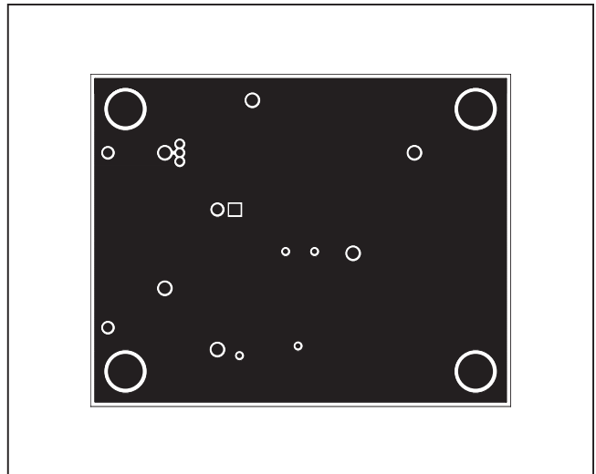
Figure 4. MAX16977 EV Kit PCB Layout—Layer 2
