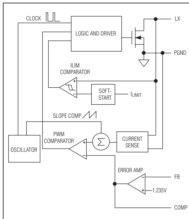
Figure 4. Step-Up Regulator Block Diagram
