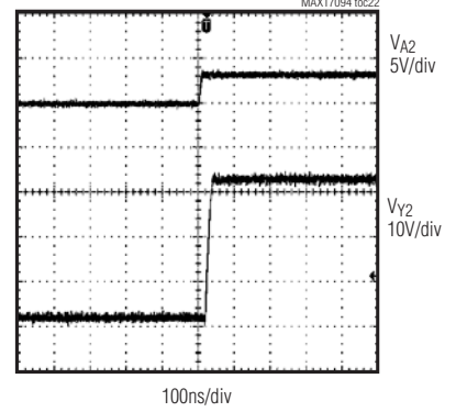
SCAN DRIVER PROPAGATION DELAY (RISING EDGE)
