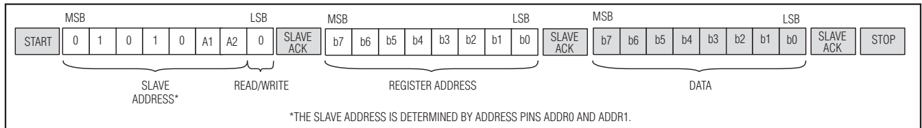
Figure 11. Write Operation
