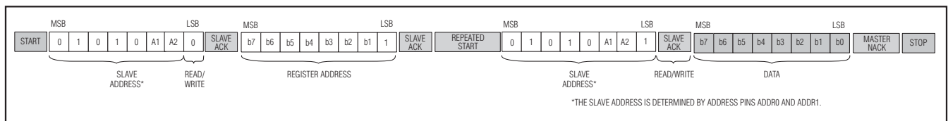
Figure 12. Read Operation
