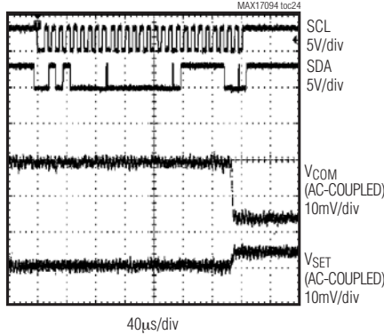
CALIBRATION SIGNAL LSB DOWNWARD STEP RESPONSE
