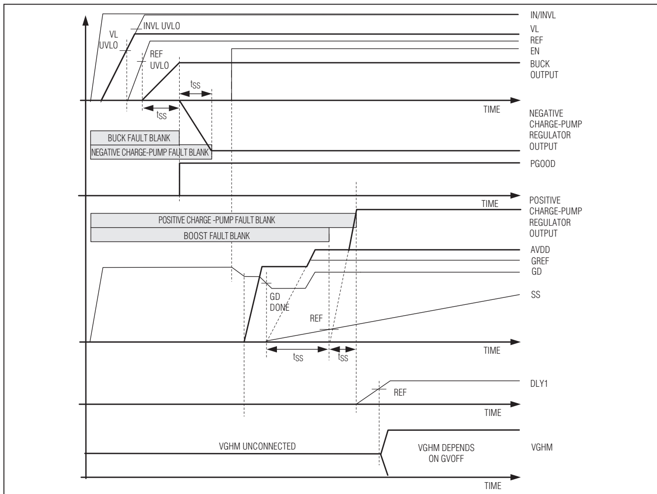
Figure 7. Power-Up Sequence
