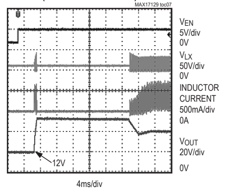
STARTUP WAVEFORMS (BRIGHTNESS = 100%)
