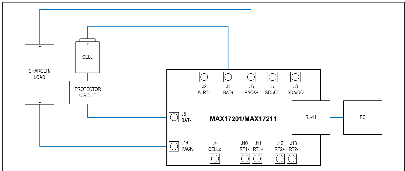
Figure 1. MAX17201/MAX17211 Board Connections
